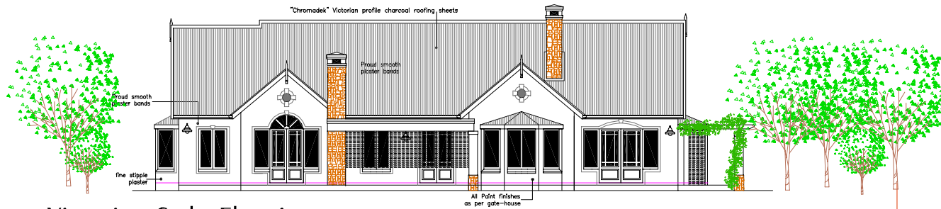
VICTORIAN Style Elevation
